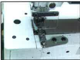
Stitch length adjustment by push button
