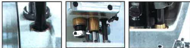
Oil seal in bush for needle bar and presser foot bar to stop oil leak
